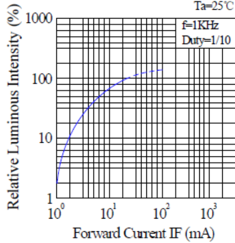
Luminous Intensity & Forward Current
