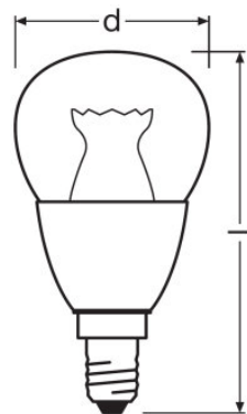
PARATHOM CL P 40 270° ADV 6 W/827 E14 N/A
