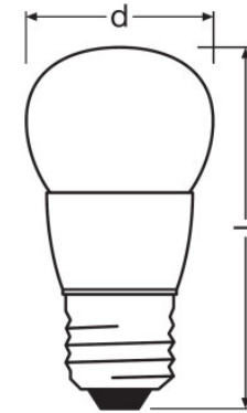
PARATHOM CL P 25 270° ADV 3.2 W/827 E27 N/A, PARATHOM CL P 40 270° ADV 6 W/827 E27 N/A
